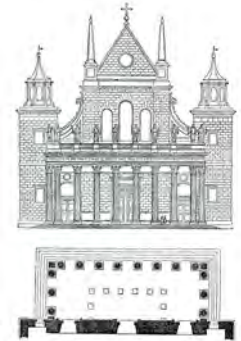
PLAN AND ELEVATION OF THE PORTION OF OLD ST. PAUL'S, THE PLAN OF THE PORTION OF ST. WENDEL'S CHURCH IN DOTTED LINES, IN ORDER TO GIVE AN IDEA OF THE WHOLE.
