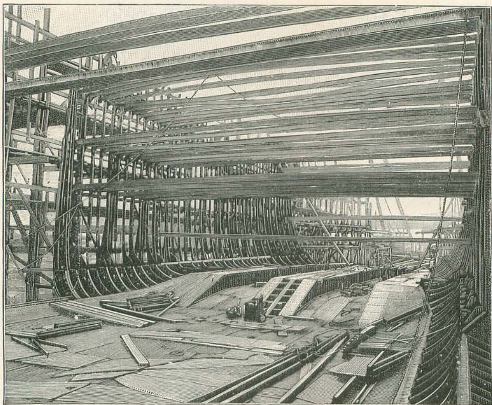
THE SKELETON OF THE "DEUTSCHLAND."
