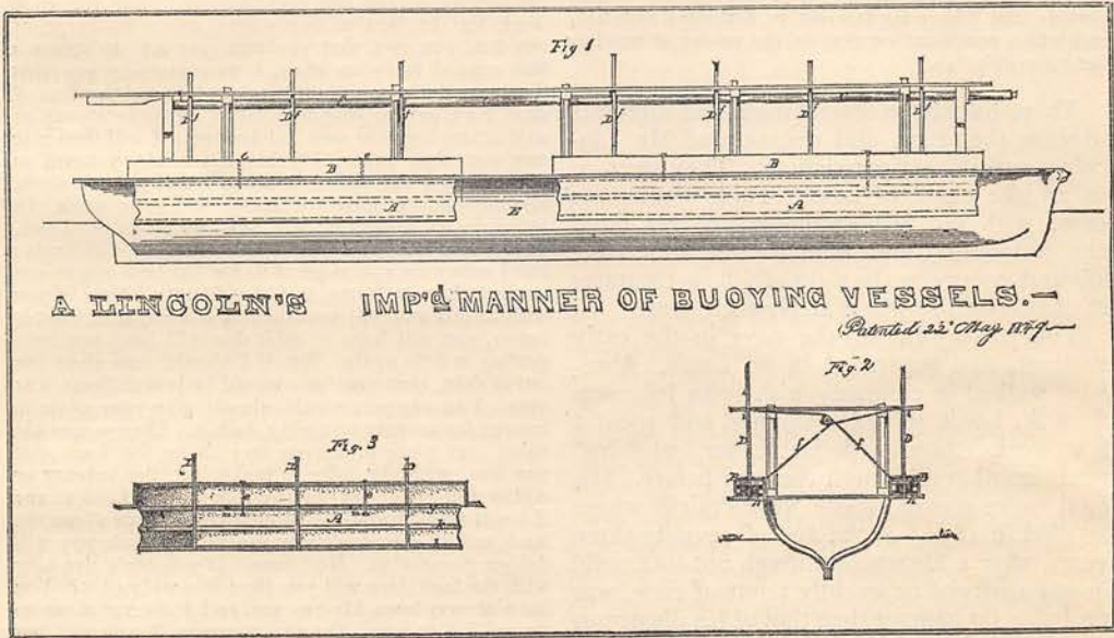
REDUCED FAC-SIMILES OF DRAWINGS IN PATENT OFFICE.
