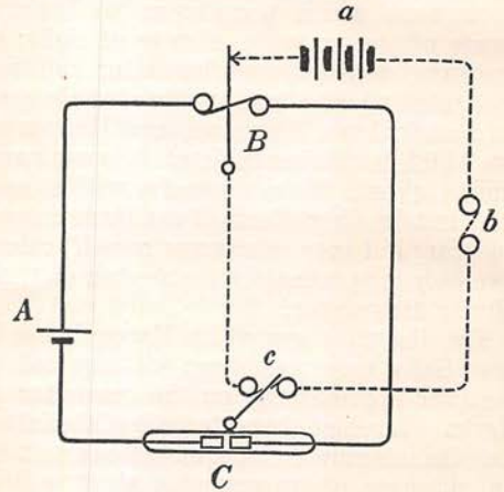
FIG. 6. MARCONI'S RECEIVER. A—Desiccator. a—Battery. B—Relay. b—Morse indicator. C—Coherer. c—Ticker.
