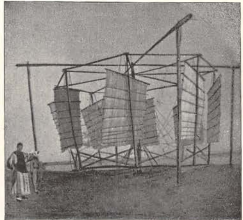
WINDMILLS AT TONG-KU FOR RAISING SALT WATER.
