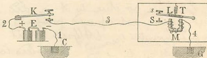
DIAGRAM ILLUSTRATING THE PRINCIPLE OF THE MODERN TELEGRAPH.
