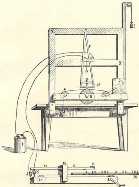
DIAGRAM OF MORSE'S EXPERIMENTAL INSTRUMENT, 1837.
